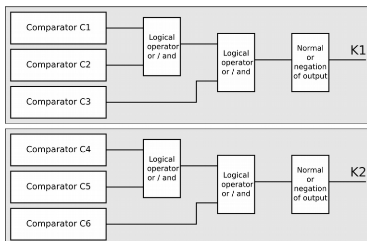
Picture 8. Comparators and logic functions
