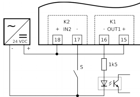
Picture 7. Connection of PLA33 input and output
