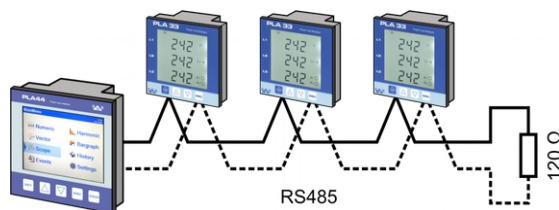
Picture 6: RS485 interface connection
