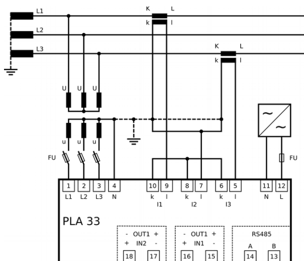
Picture 5: Connection at medium voltage network
